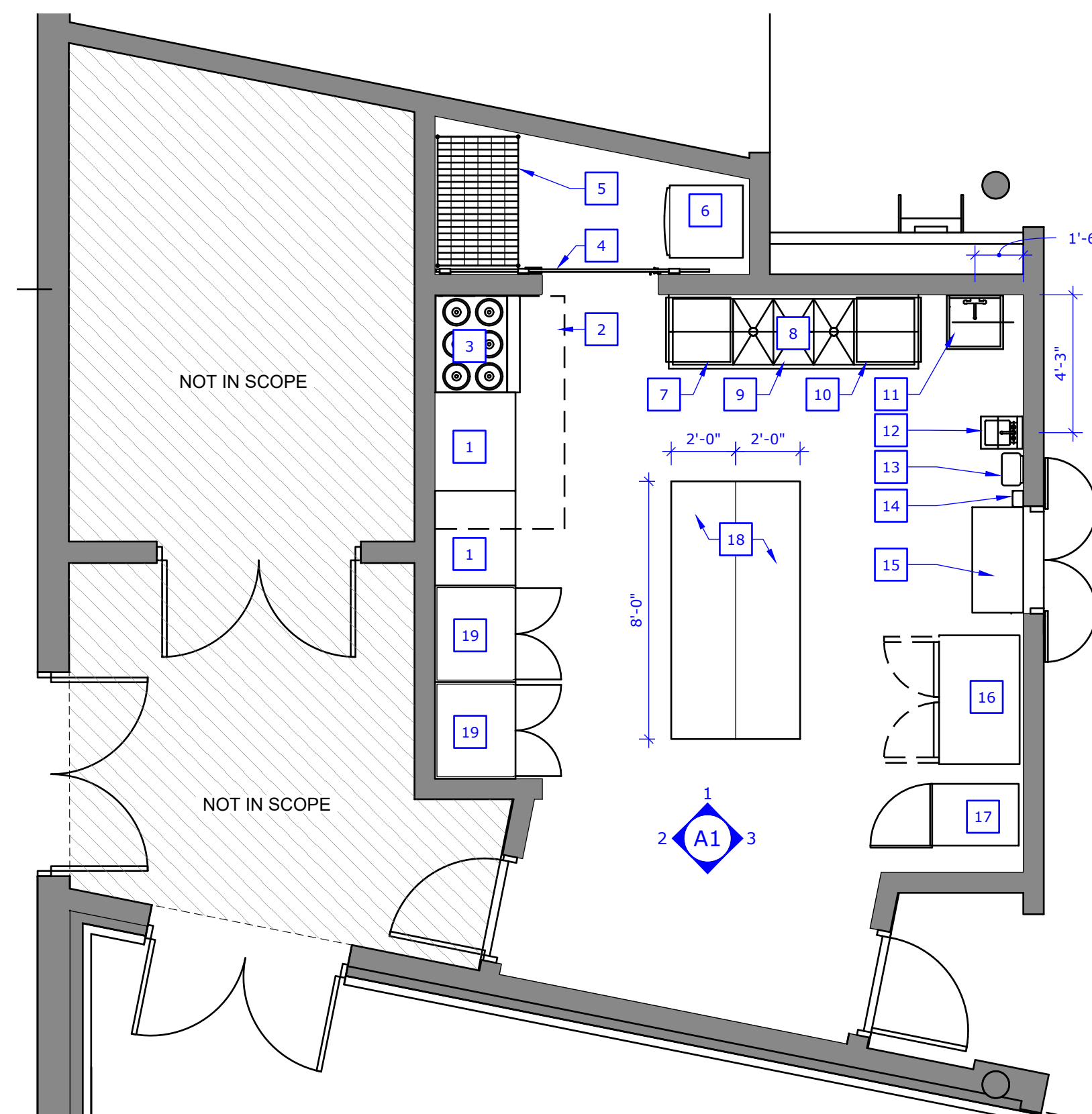
2 FLOOR PLAN - NEW WORK SCALE :: 1/4" = 1' - 0"
