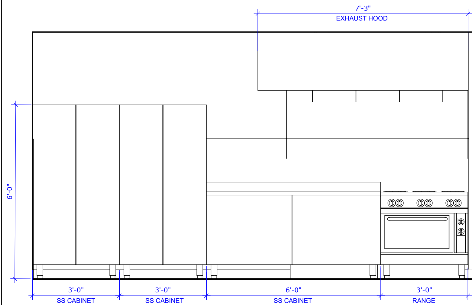
2 NORTH ELEVATION - RANGE / OVEN SCALE :: 1/4" = 1' - 0"
