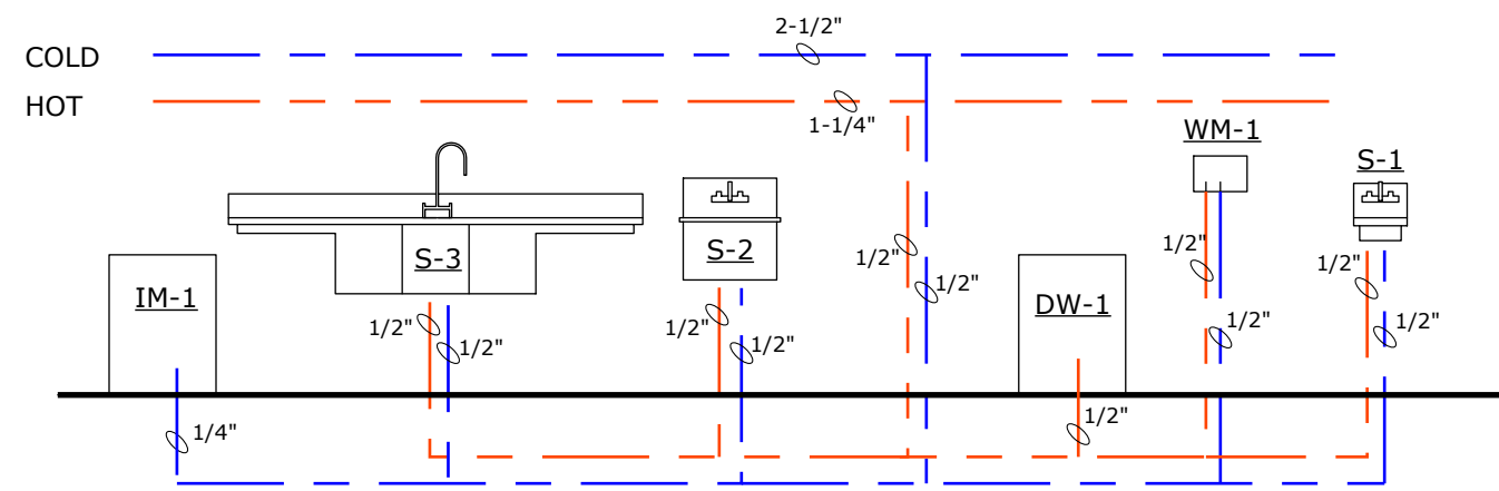
3 PLUMBING SUPPLY DIAGRAM SCALE :: 1/4" = 1' - 0"
