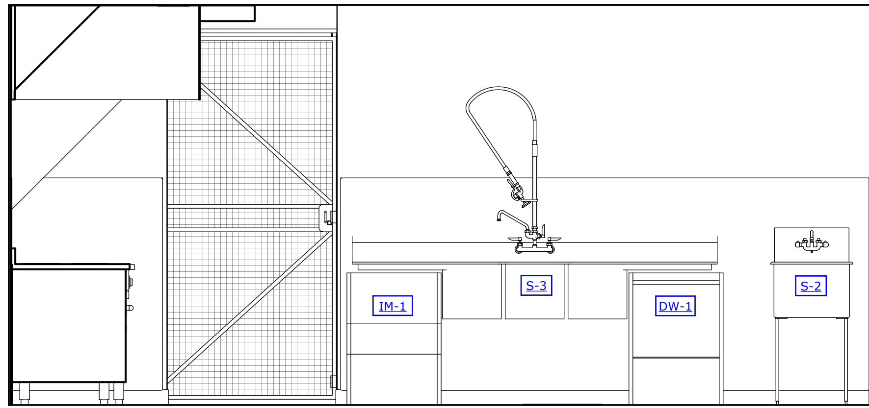
1 EAST ELEVATION - SINKS SCALE :: 1/4" = 1' - 0"
