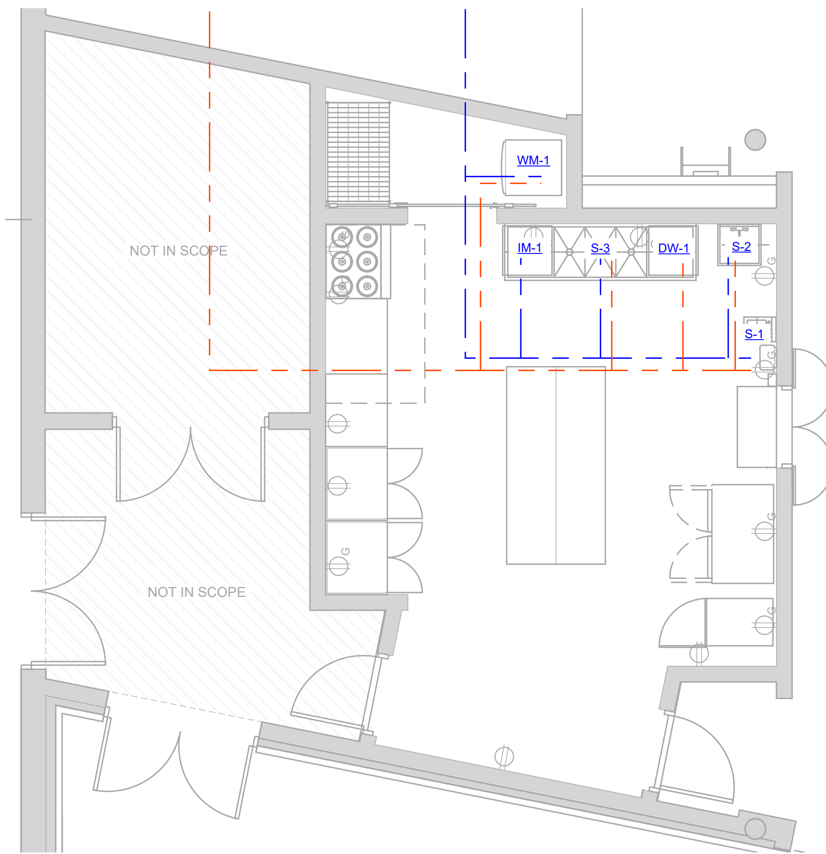
3 PLUMBING WATER SERVICE PLAN SCALE :: 1/4" = 1' - 0"
