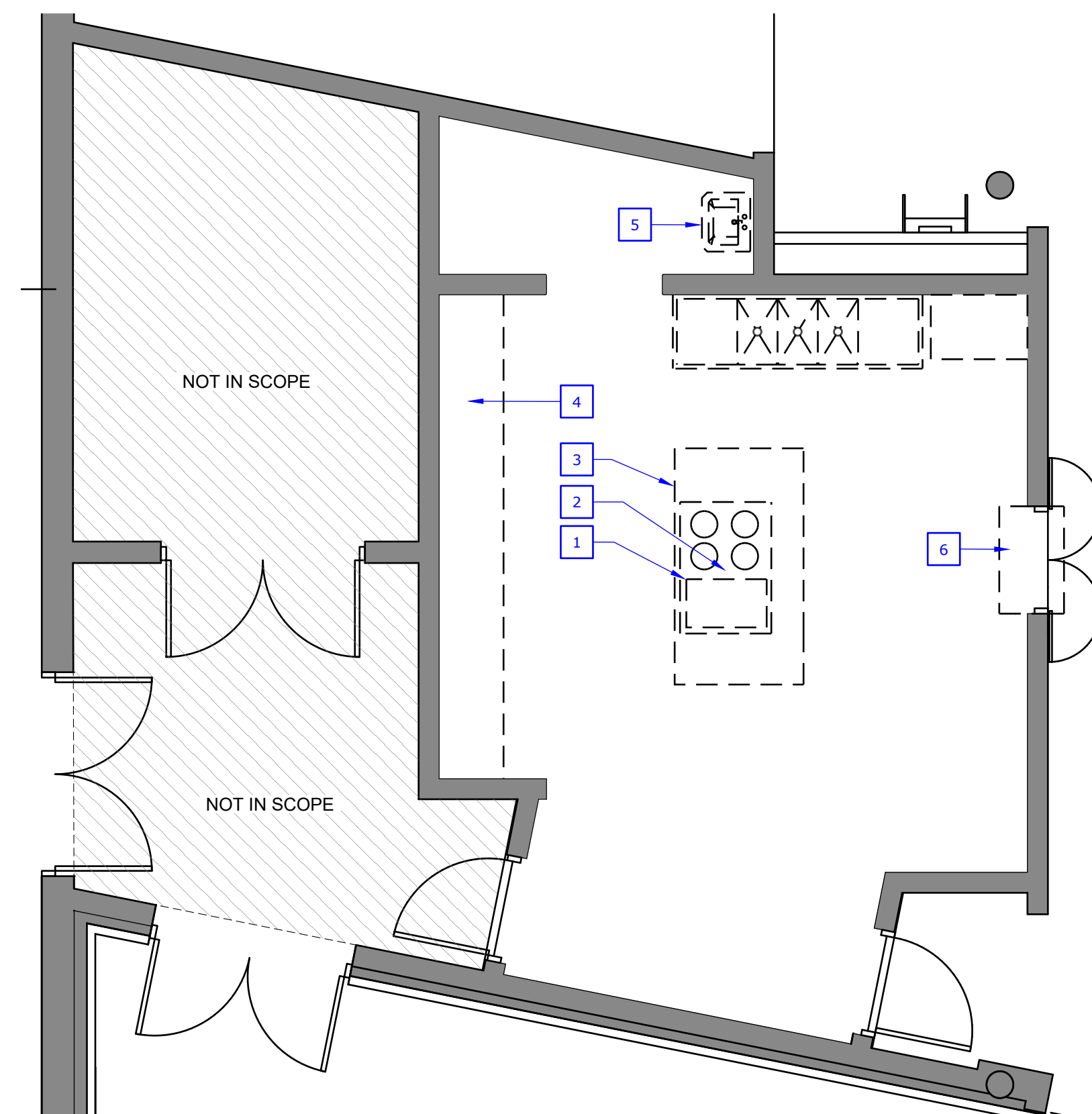
1 FLOOR PLAN - DEMOLITION SCALE :: 1/4" = 1' - 0"
