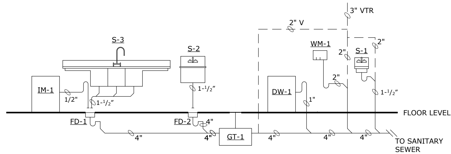
4 PLUMBING WASTE & VENT DIAGRAM SCALE :: 1/4" = 1' - 0"
