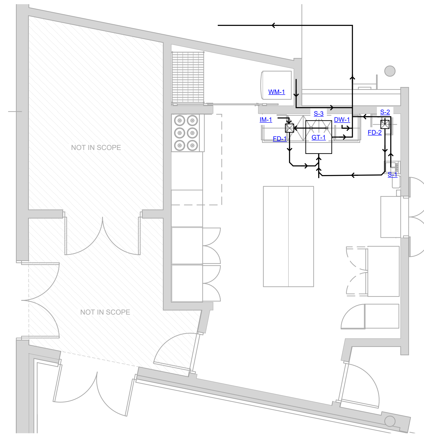
1 PLUMBING SANITARY PLAN SCALE :: 1/4" = 1' - 0"
