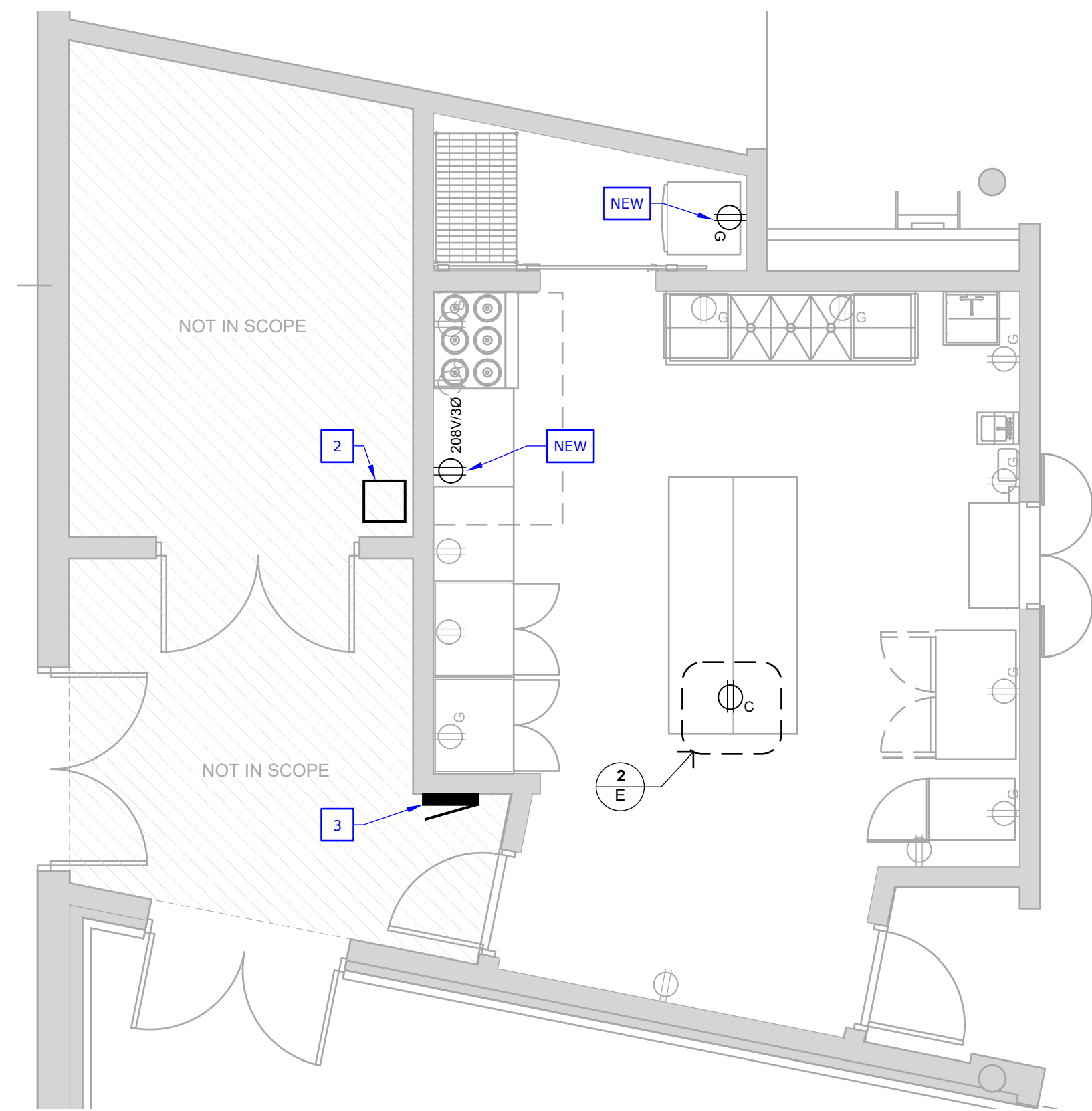
1 ELECTRICAL PLAN SCALE :: 1/4" = 1' - 0"
